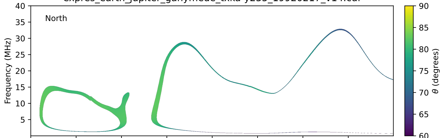
expres_earth_jupiter_ganymede_txka-y235_19920217_v14.cdf
