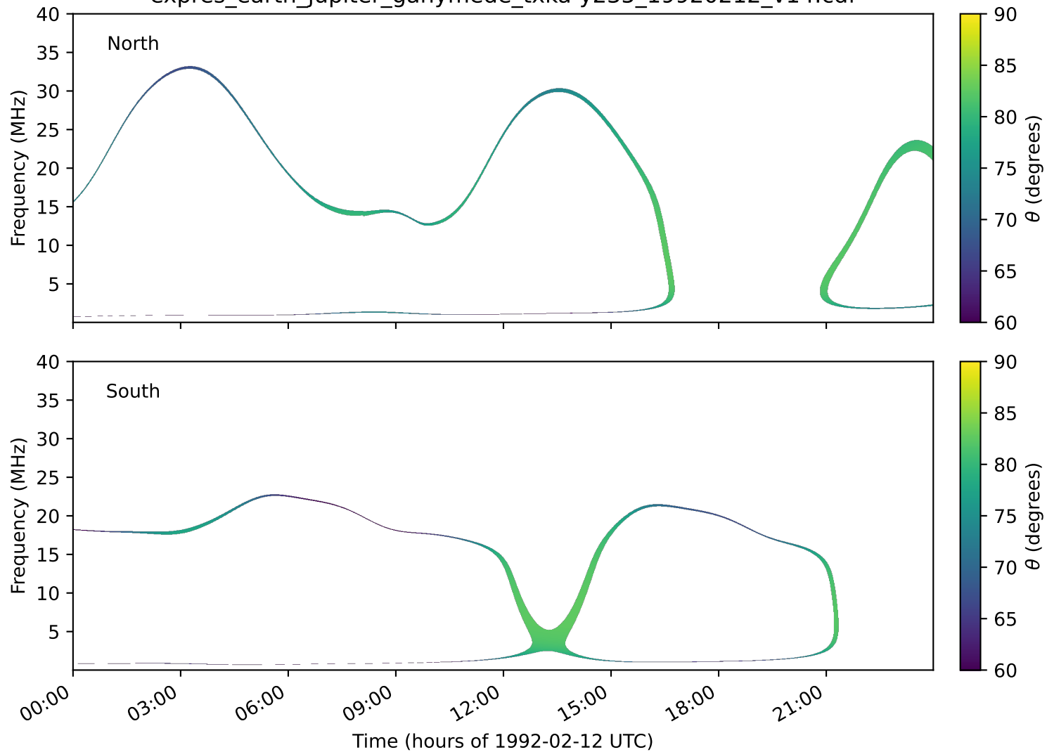
expres_earth_jupiter_ganymede_txka-y235_19920212_v14.cdf
