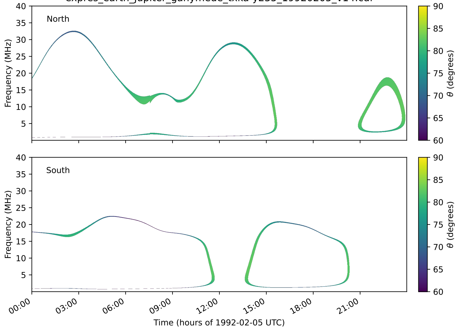
expres_earth_jupiter_ganymede_txka-y235_19920205_v14.cdf
