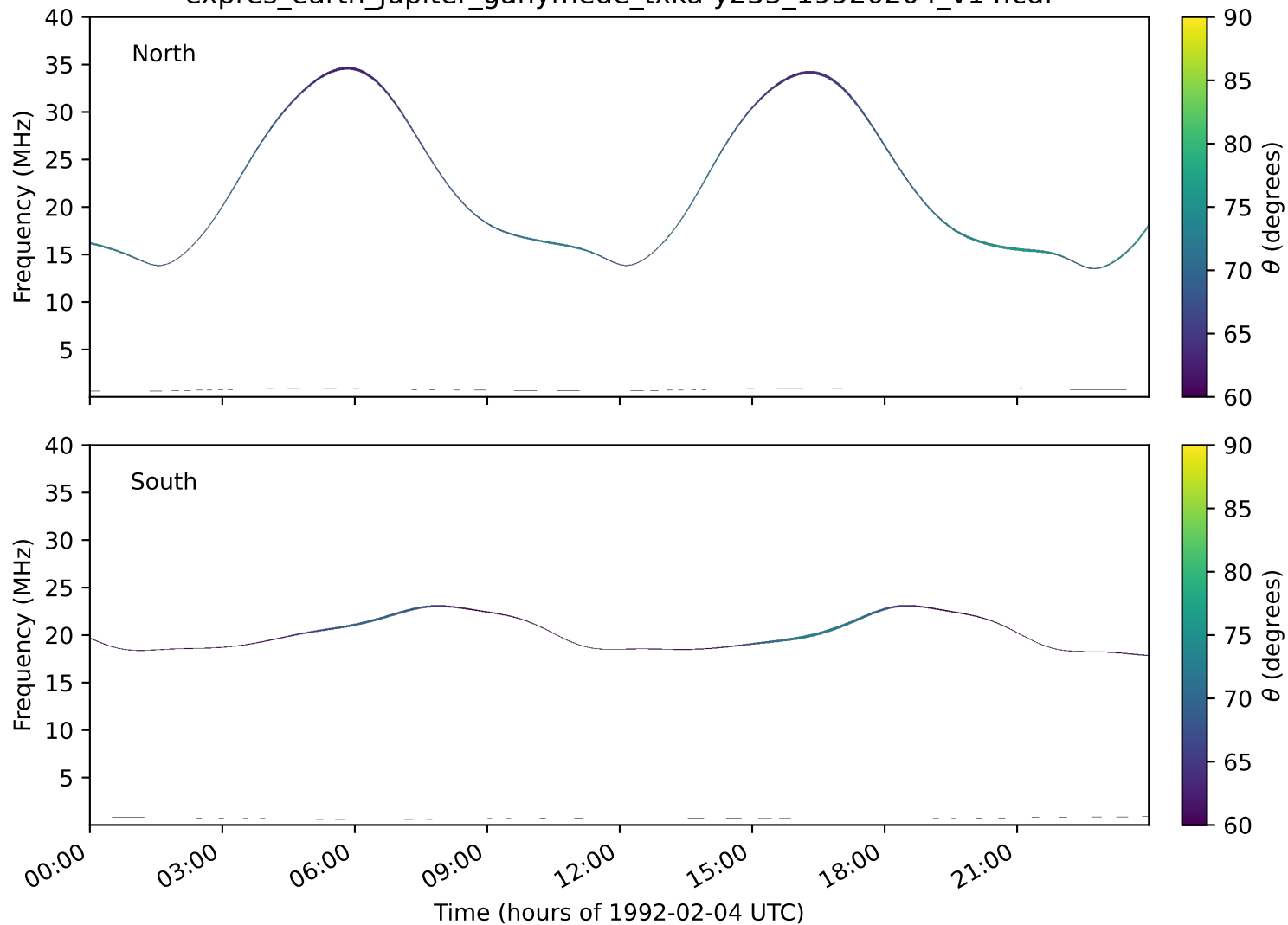
expres_earth_jupiter_ganymede_txka-y235_19920204_v14.cdf
