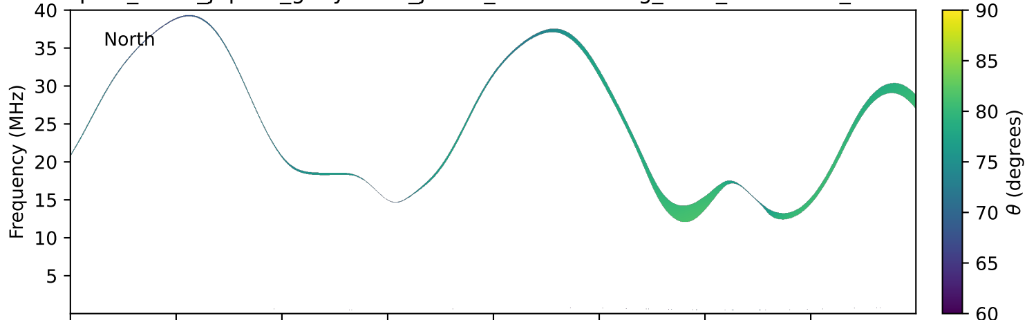
expres_earth_jupiter_ganymede_jrm33_lossc-wid1deg_3kev_19920212_v11.cdf
