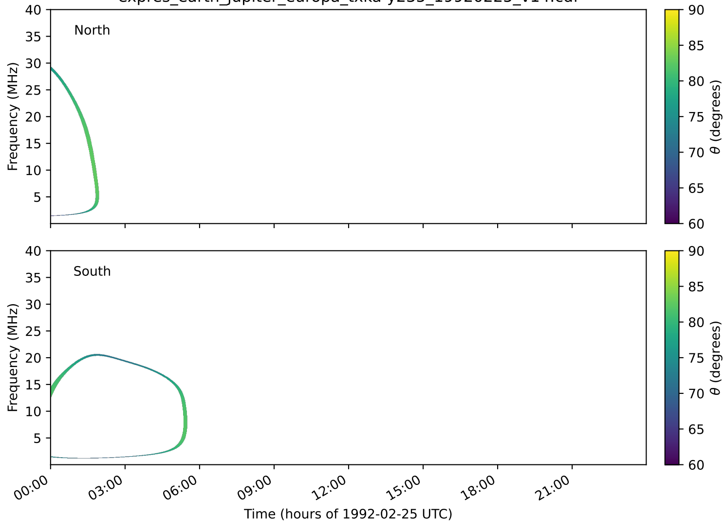
expres_earth_jupiter_europa_txka-y235_19920225_v14.cdf
