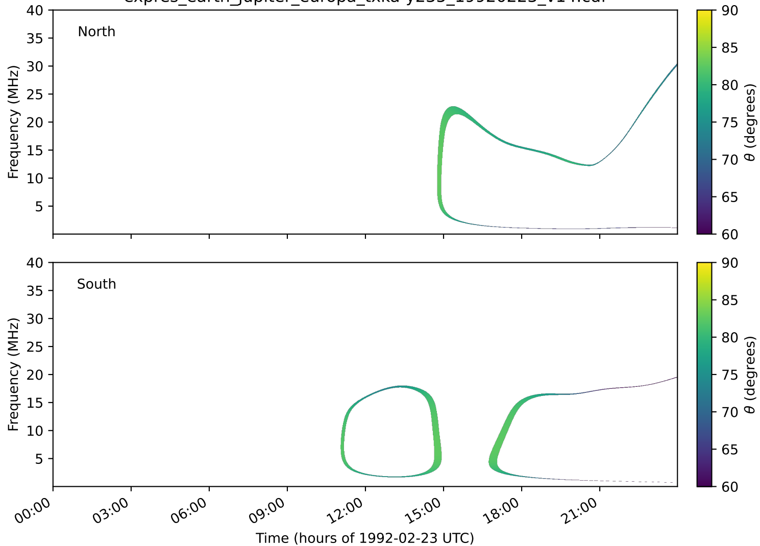
expres_earth_jupiter_europa_txka-y235_19920223_v14.cdf
