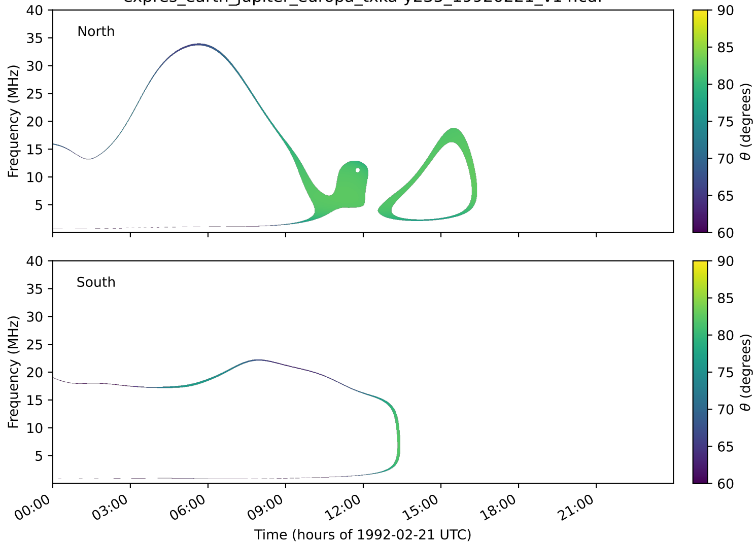
expres_earth_jupiter_europa_txka-y235_19920221_v14.cdf
