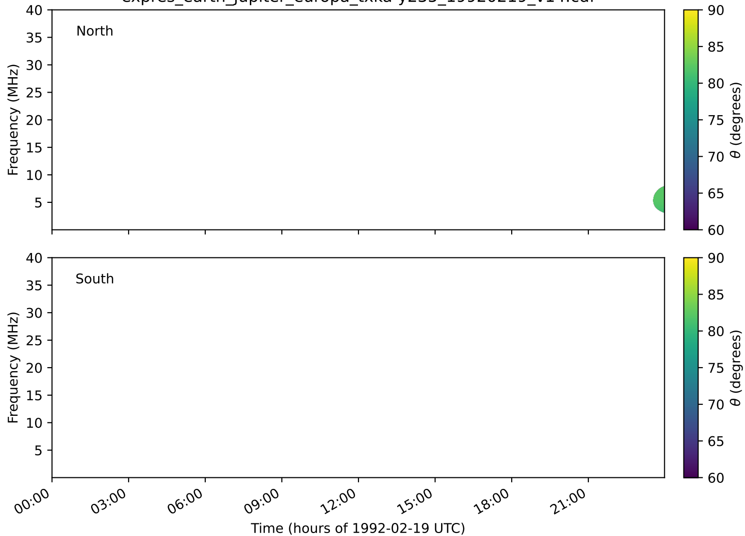
expres_earth_jupiter_europa_txka-y235_19920219_v14.cdf
