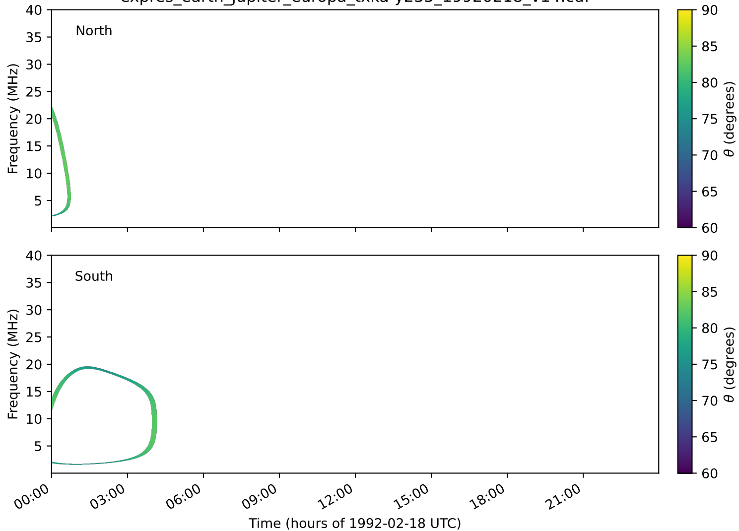
expres_earth_jupiter_europa_txka-y235_19920218_v14.cdf
