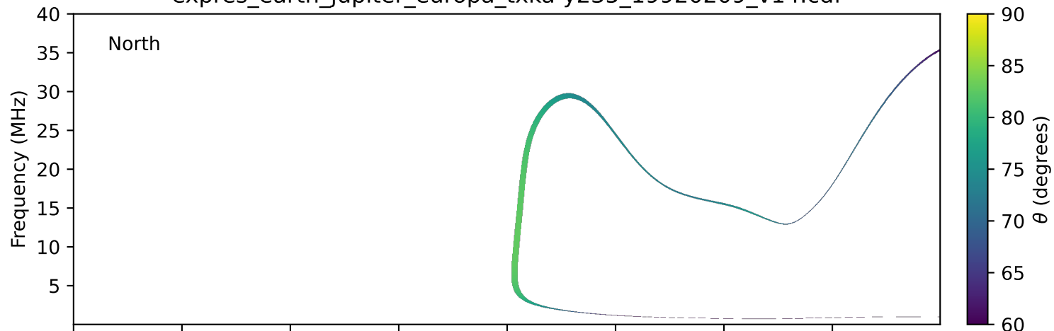
expres_earth_jupiter_europa_txka-y235_19920209_v14.cdf
