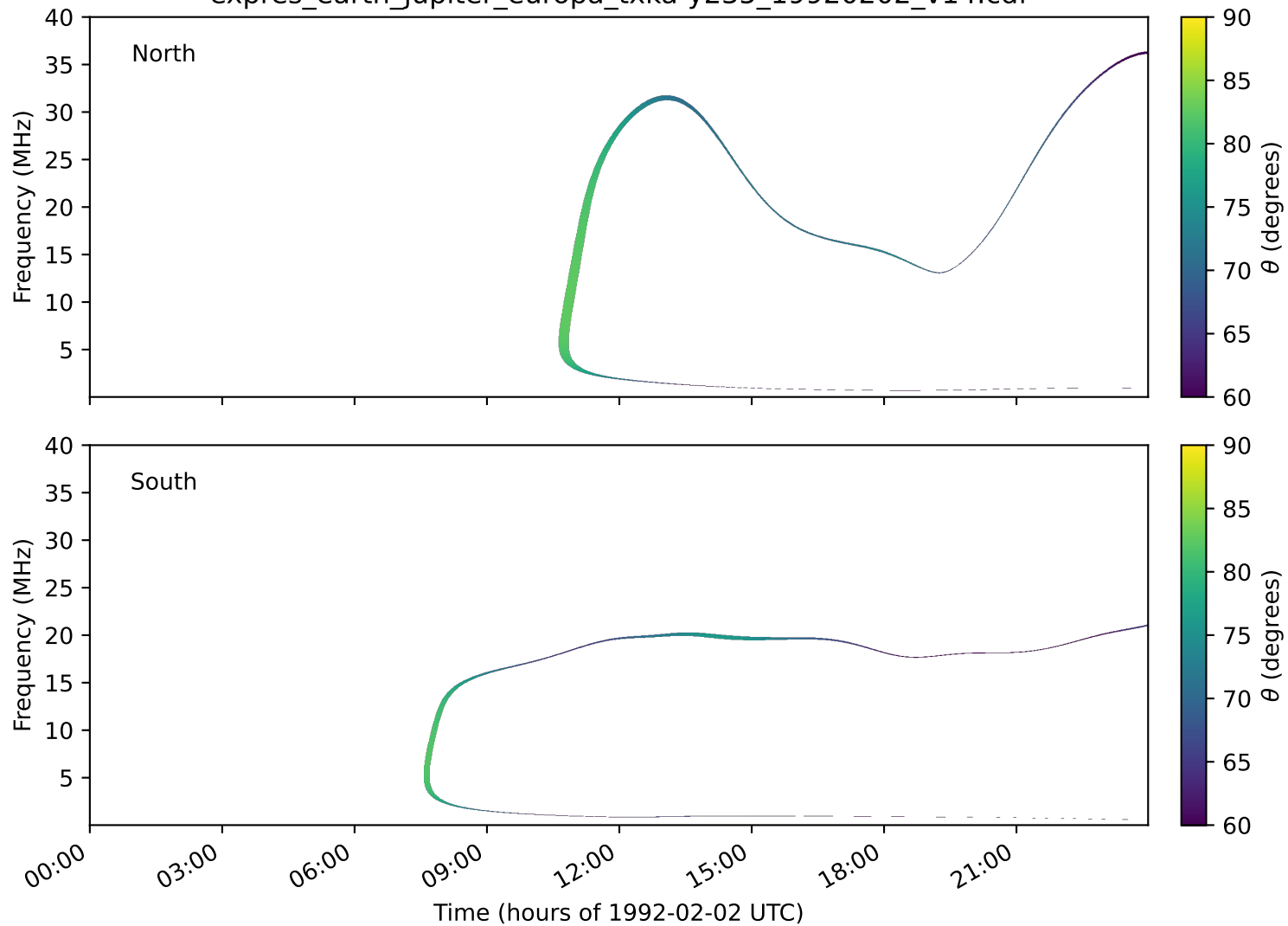
expres_earth_jupiter_europa_txka-y235_19920202_v14.cdf
