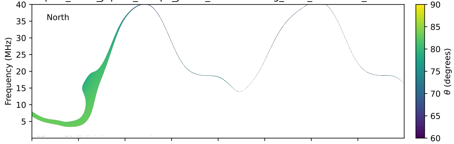
expres_earth_jupiter_europa_jrm33_lossc-wid1deg_3kev_19920213_v11.cdf
