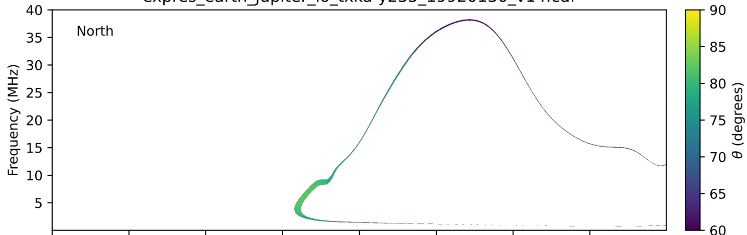
expres_earth_jupiter_io_txka-y235_19920130_v14.cdf
