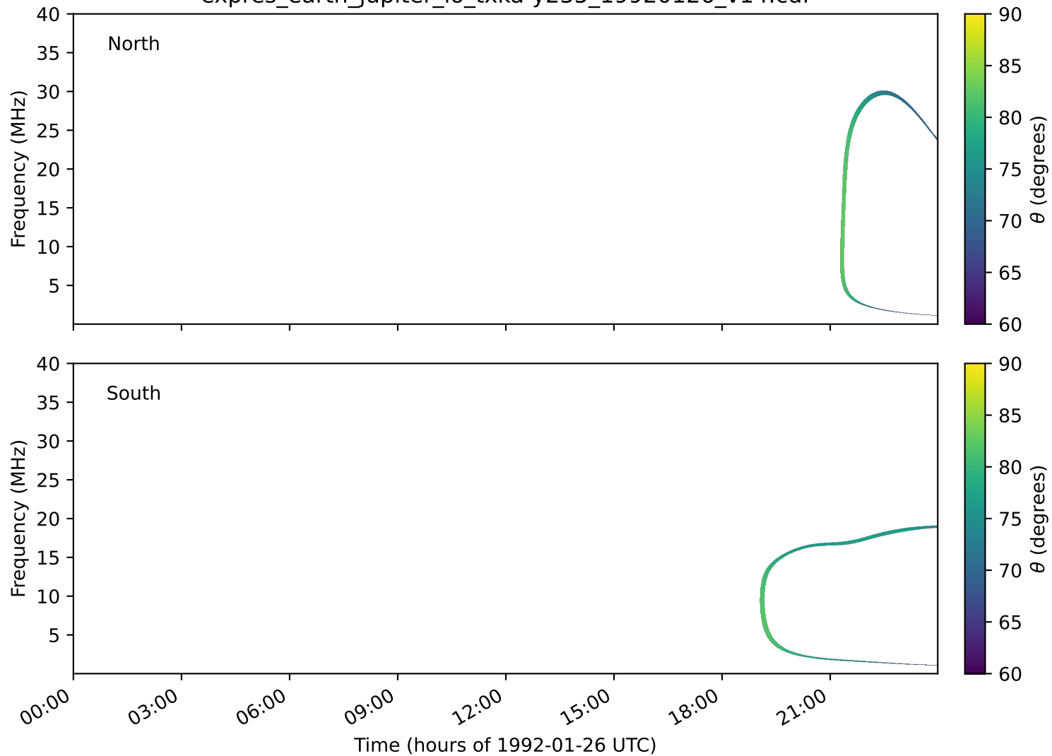
expres_earth_jupiter_io_txka-y235_19920126_v14.cdf
