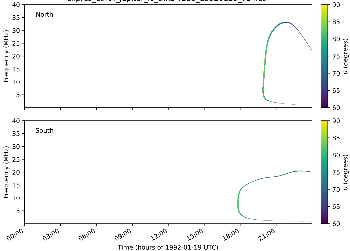
expres_earth_jupiter_io_txka-y235_19920119_v14.cdf
