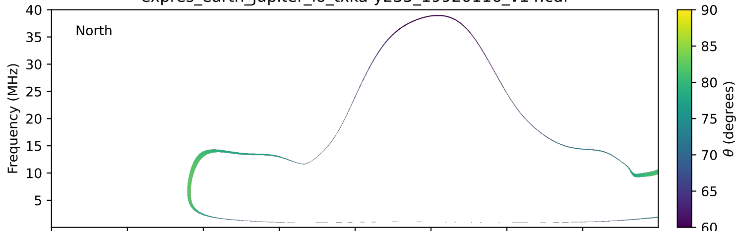
expres_earth_jupiter_io_txka-y235_19920116_v14.cdf
