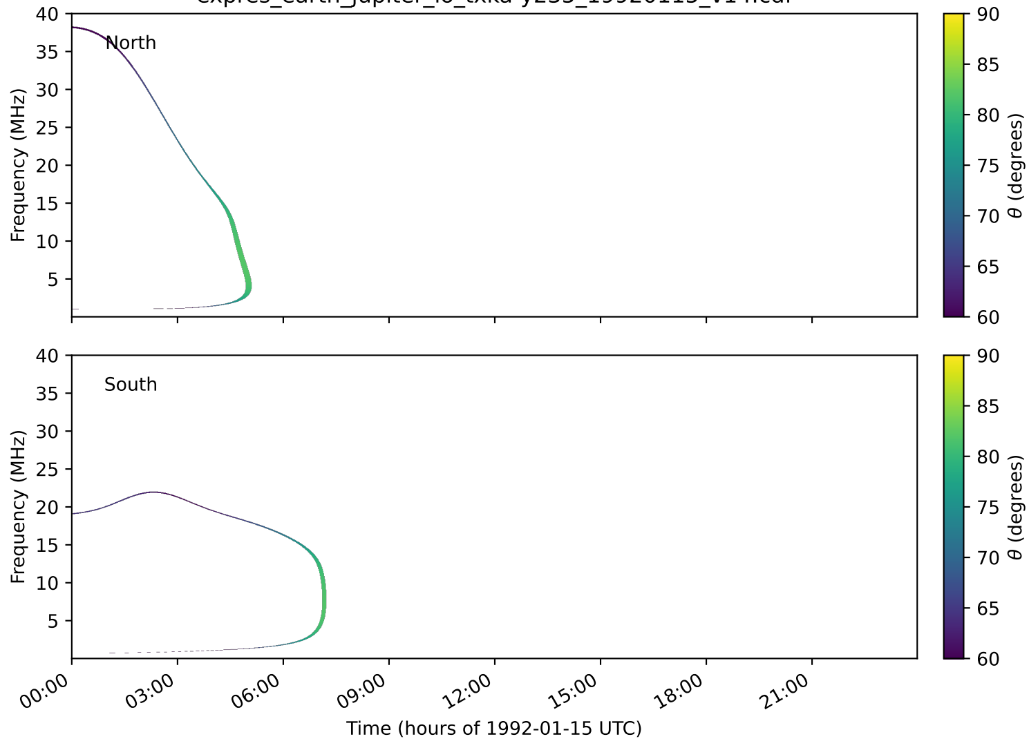
expres_earth_jupiter_io_txka-y235_19920115_v14.cdf
