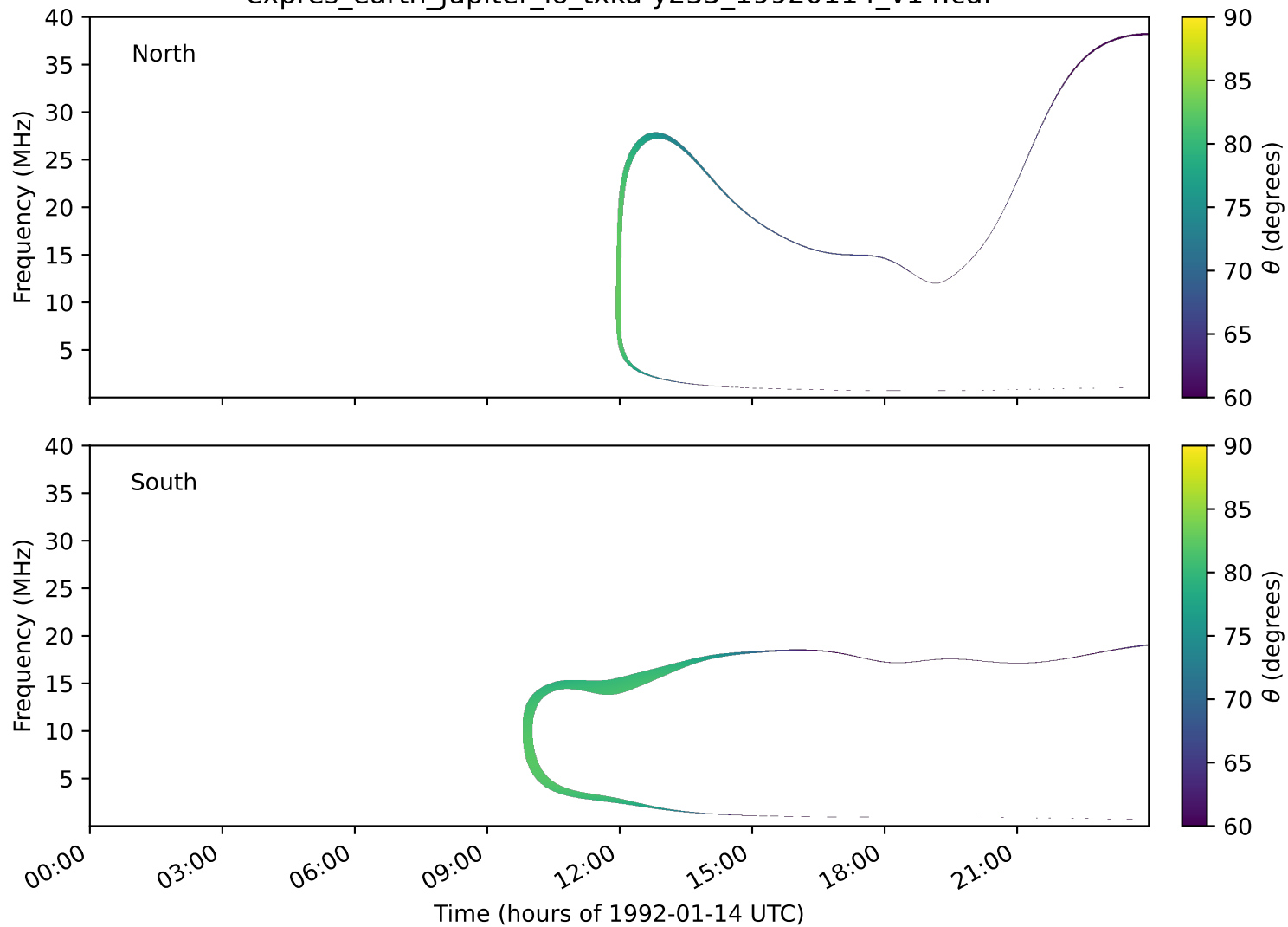
expres_earth_jupiter_io_txka-y235_19920114_v14.cdf
