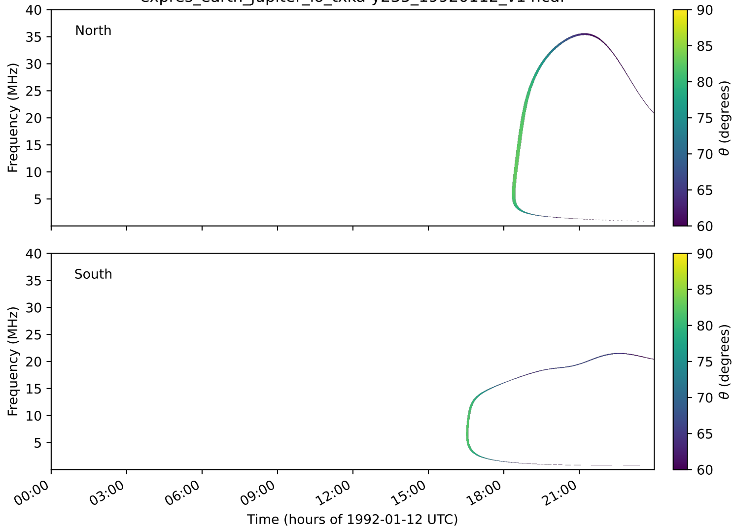
expres_earth_jupiter_io_txka-y235_19920112_v14.cdf
