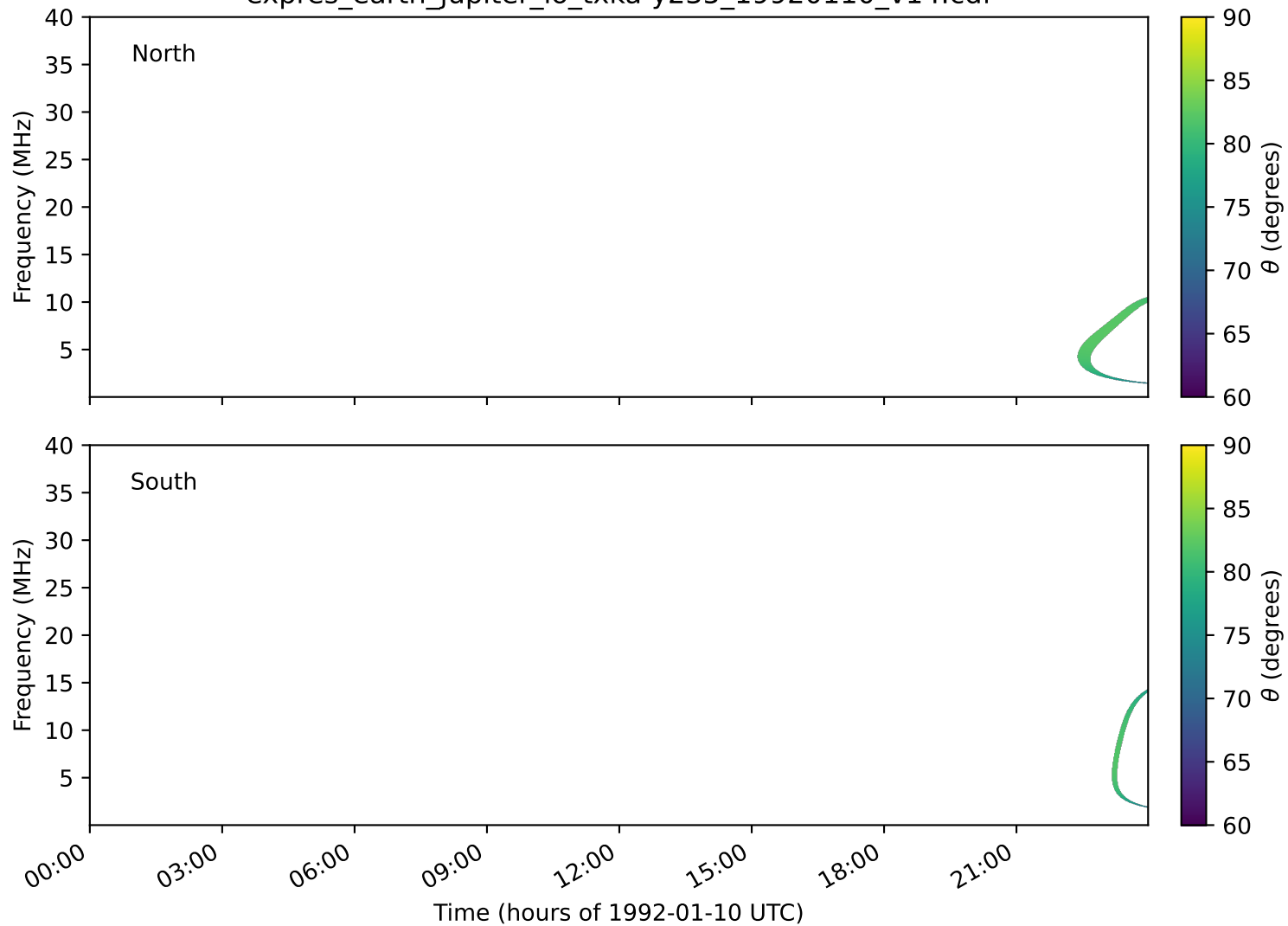
expres_earth_jupiter_io_txka-y235_19920110_v14.cdf
