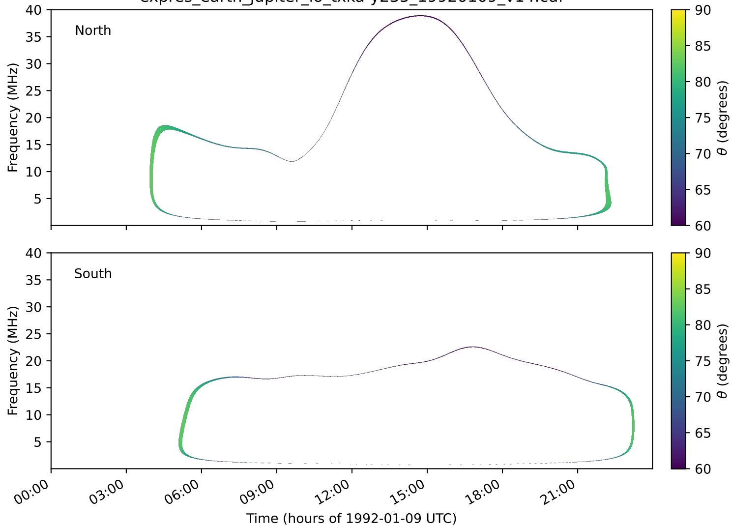
expres_earth_jupiter_io_txka-y235_19920109_v14.cdf
