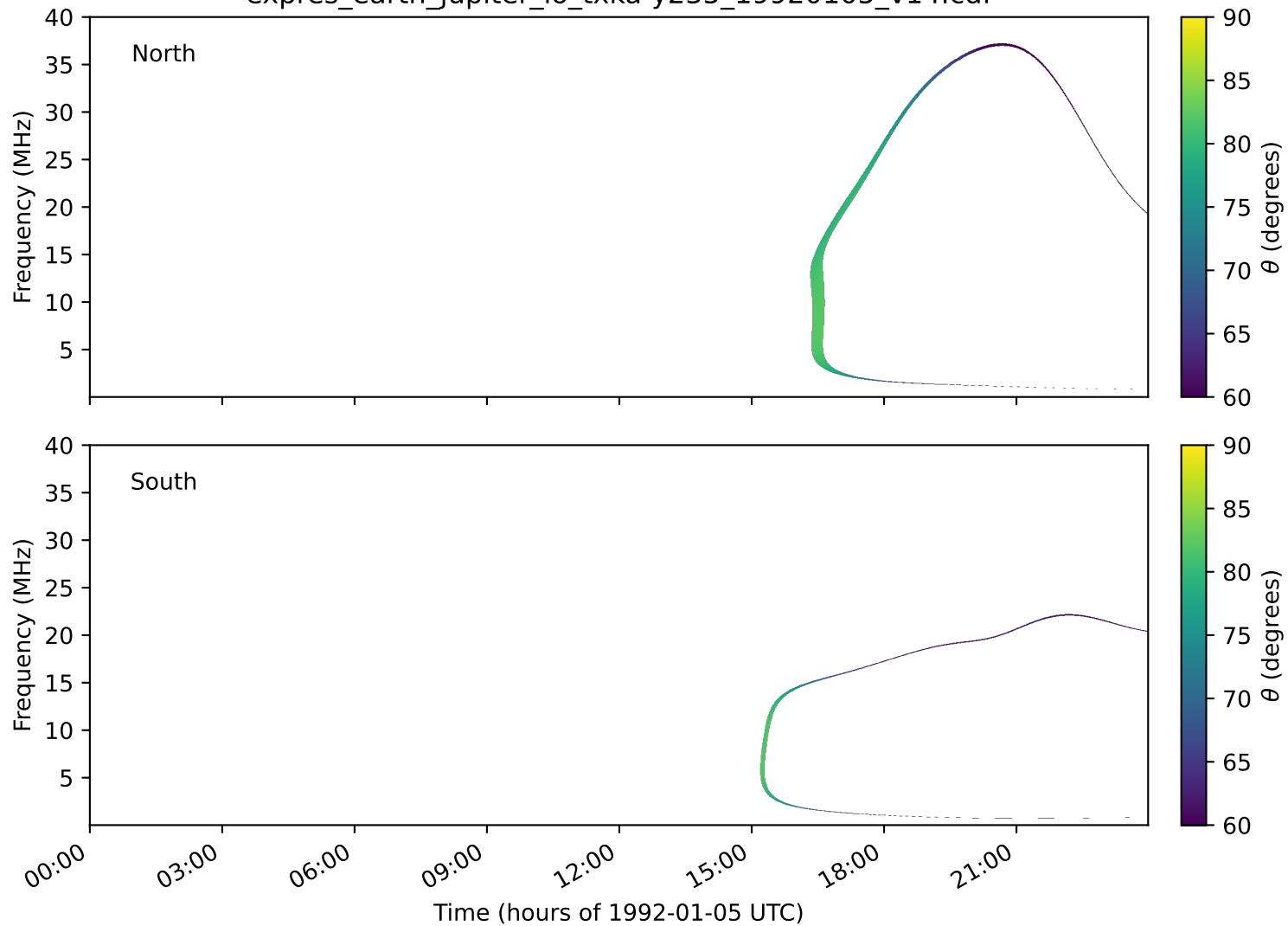
expres_earth_jupiter_io_txka-y235_19920105_v14.cdf
