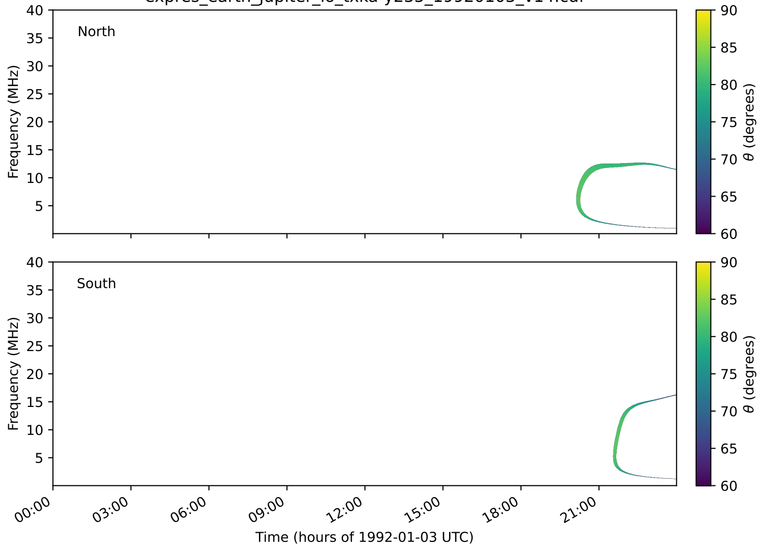
expres_earth_jupiter_io_txka-y235_19920103_v14.cdf
