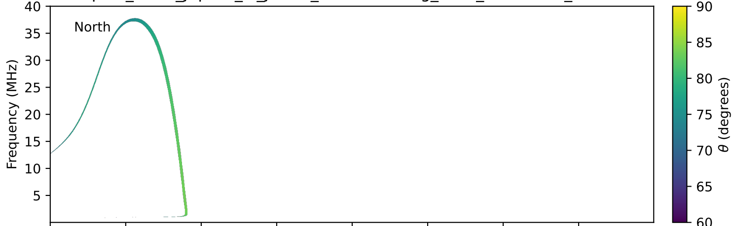
expres_earth_jupiter_io_jrm33_lossc-wid1deg_3kev_19920131_v11.cdf
