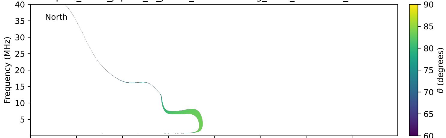
expres_earth_jupiter_io_jrm33_lossc-wid1deg_3kev_19920129_v11.cdf
