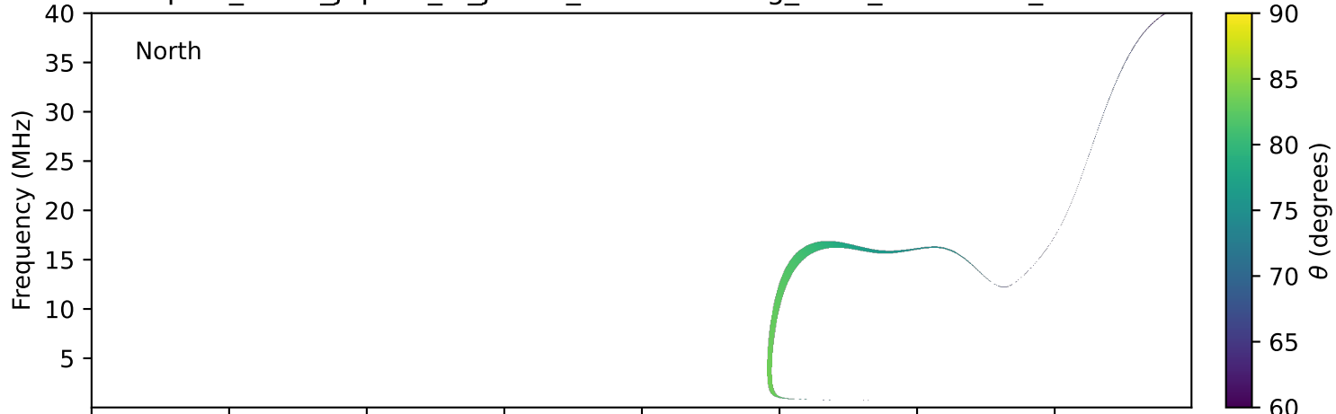
expres_earth_jupiter_io_jrm33_lossc-wid1deg_3kev_19920128_v11.cdf
