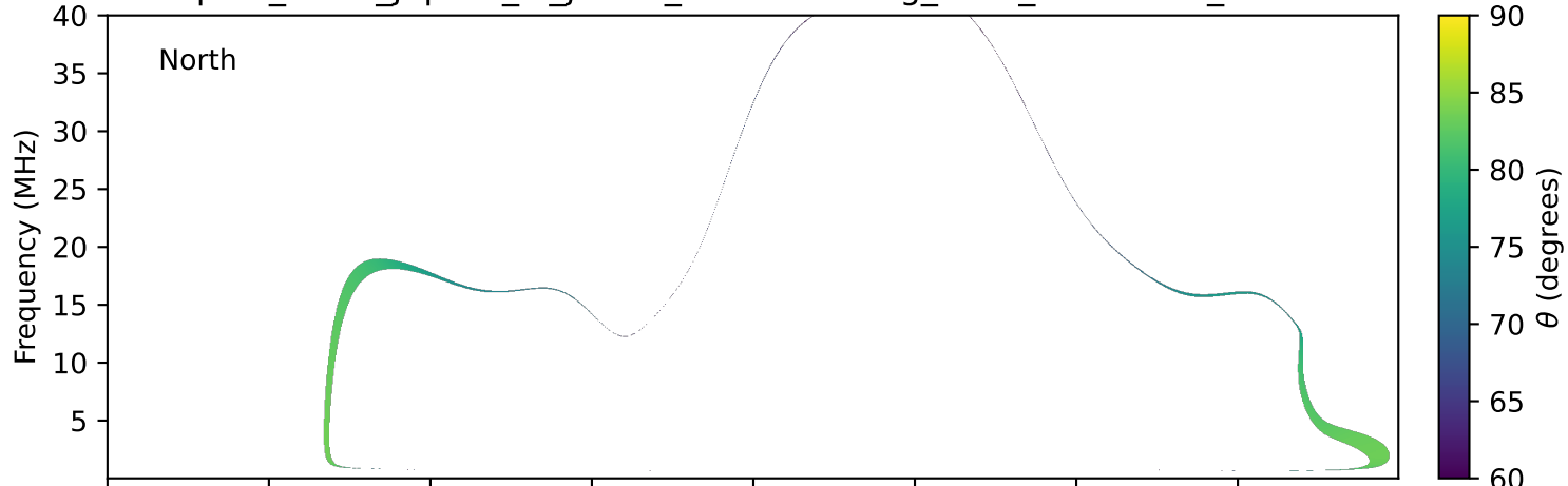
expres_earth_jupiter_io_jrm33_lossc-wid1deg_3kev_19920109_v11.cdf
