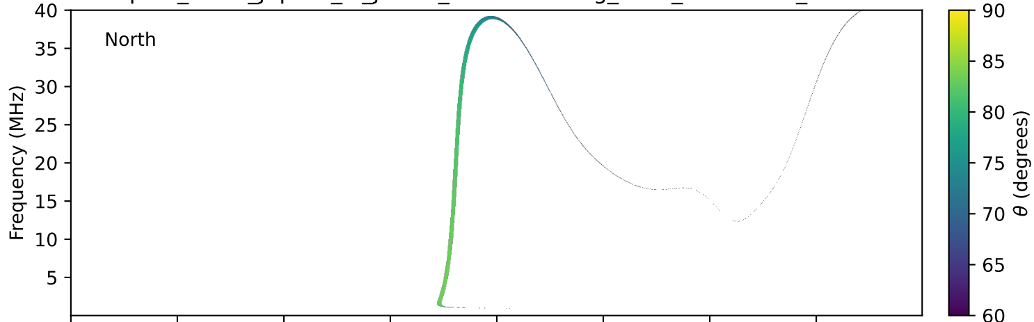
expres_earth_jupiter_io_jrm33_lossc-wid1deg_3kev_19920107_v11.cdf
