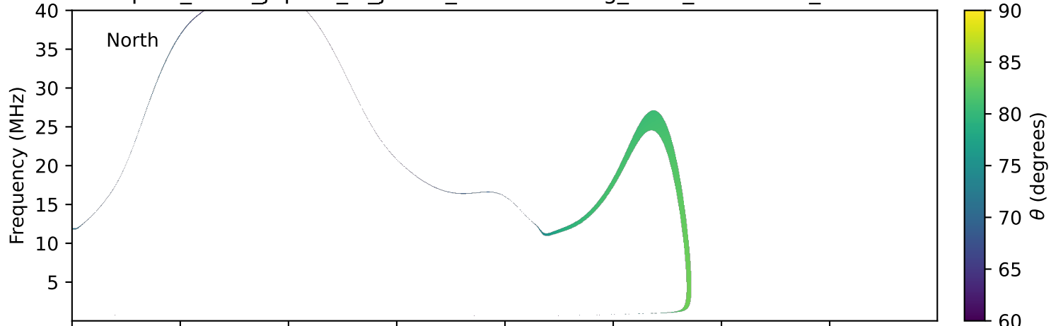
expres_earth_jupiter_io_jrm33_lossc-wid1deg_3kev_19920104_v11.cdf
