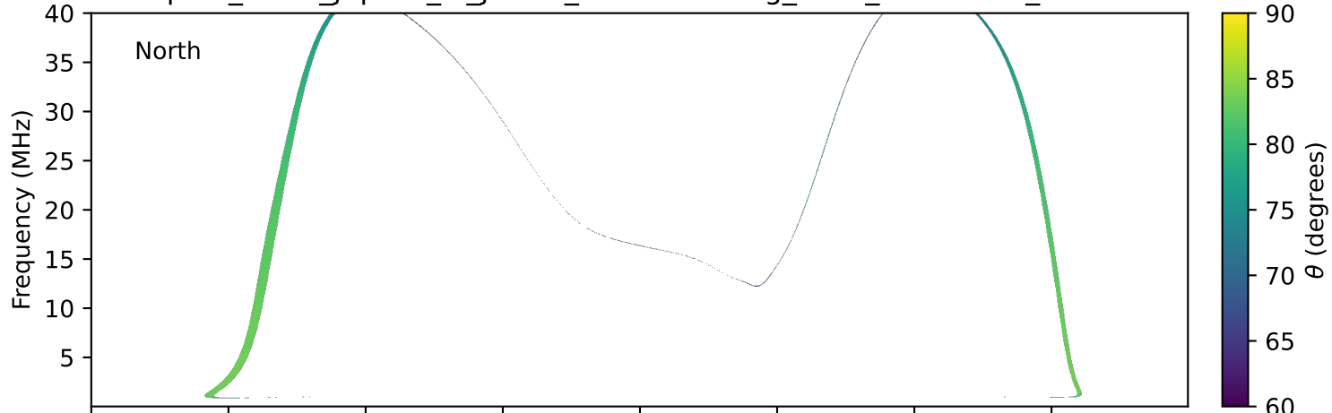
expres_earth_jupiter_io_jrm09_lossc-wid1deg_3kev_19920125_v11.cdf
