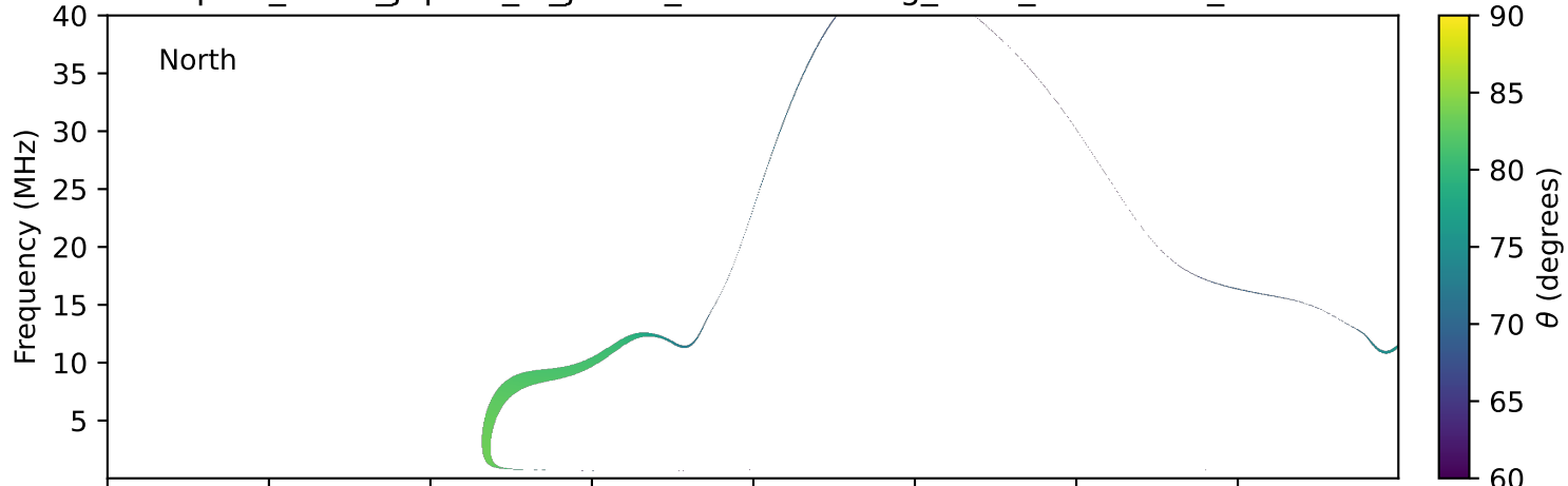
expres_earth_jupiter_io_jrm09_lossc-wid1deg_3kev_19920123_v11.cdf
