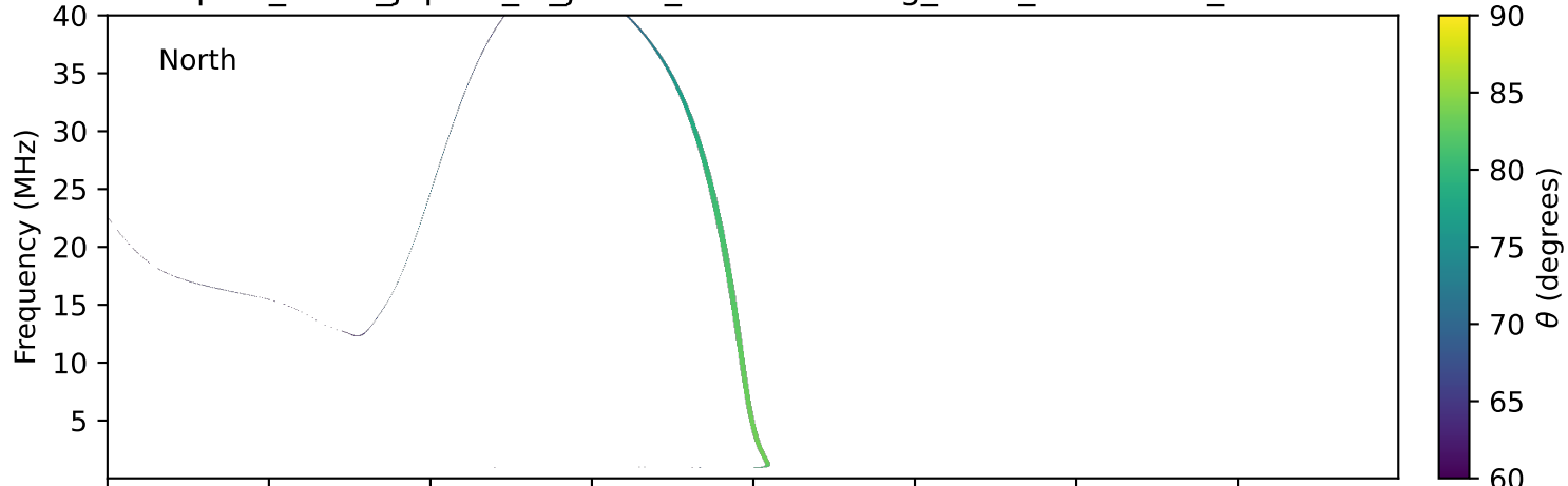
expres_earth_jupiter_io_jrm09_lossc-wid1deg_3kev_19920113_v11.cdf
