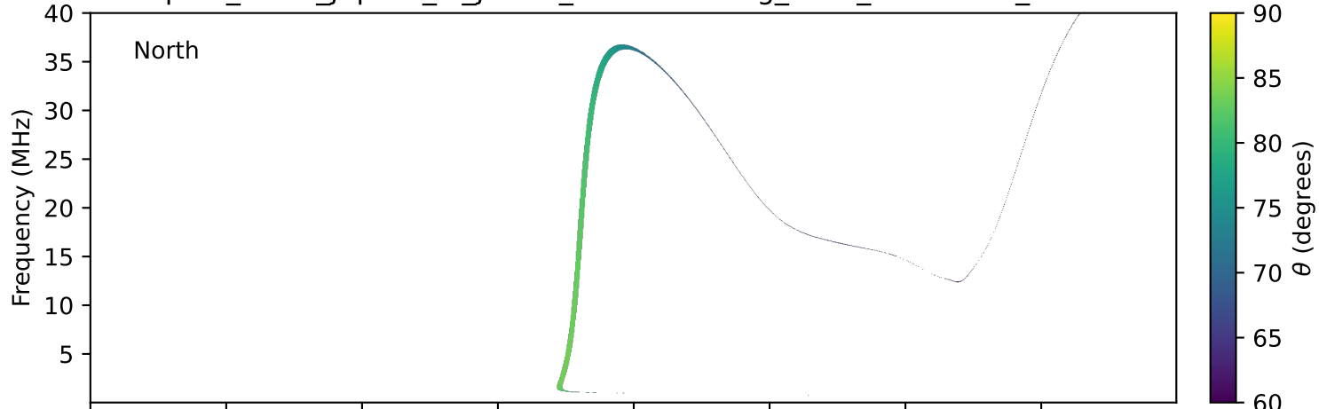
expres_earth_jupiter_io_jrm09_lossc-wid1deg_3kev_19920107_v11.cdf
