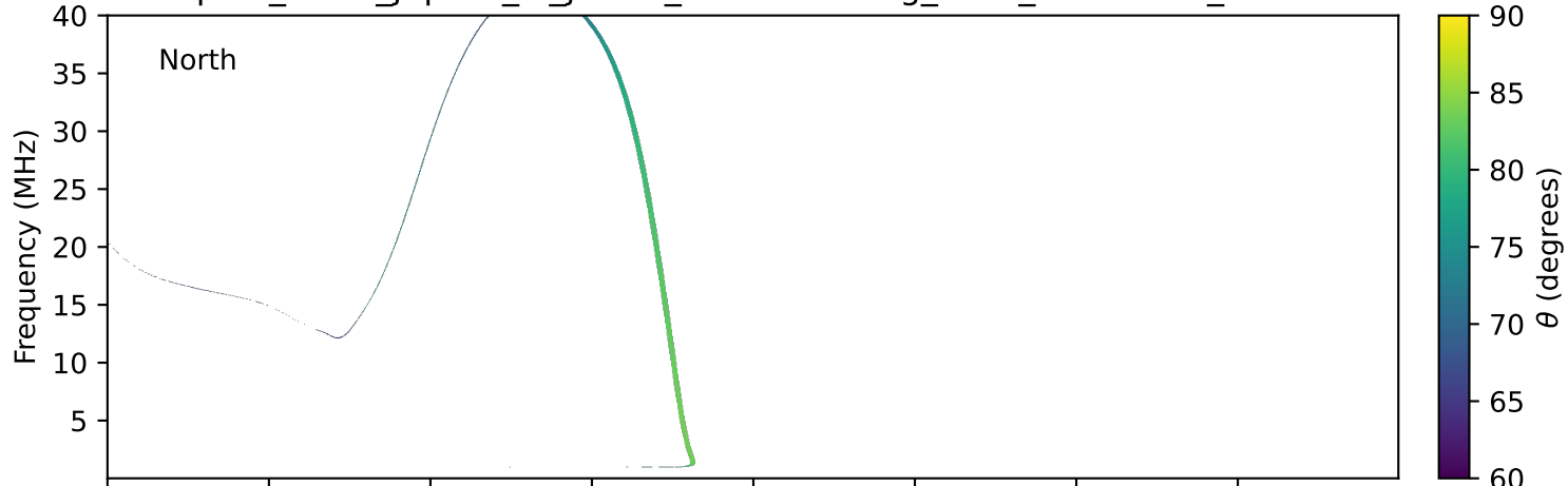
expres_earth_jupiter_io_jrm09_lossc-wid1deg_3kev_19920106_v11.cdf
