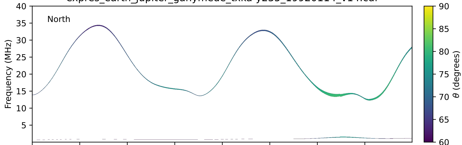
expres_earth_jupiter_ganymede_txka-y235_19920114_v14.cdf
