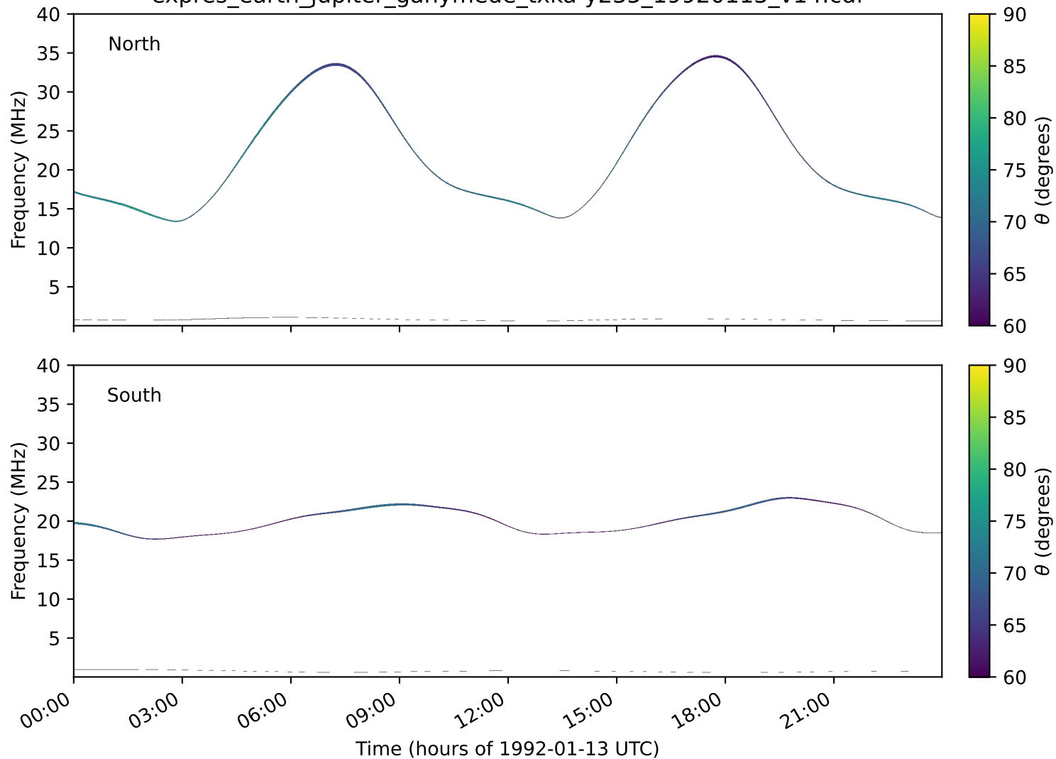
expres_earth_jupiter_ganymede_txka-y235_19920113_v14.cdf
