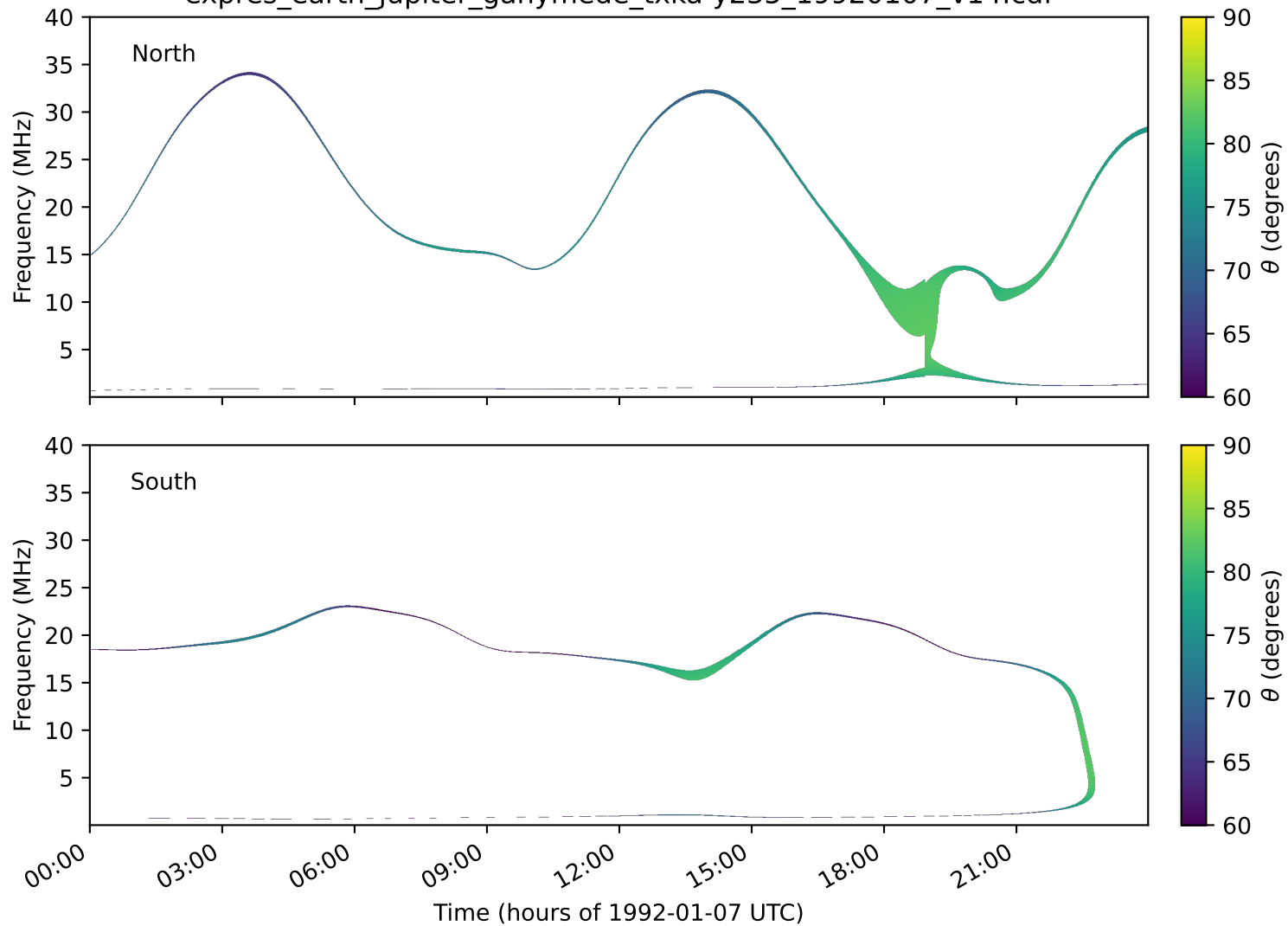
expres_earth_jupiter_ganymede_txka-y235_19920107_v14.cdf
