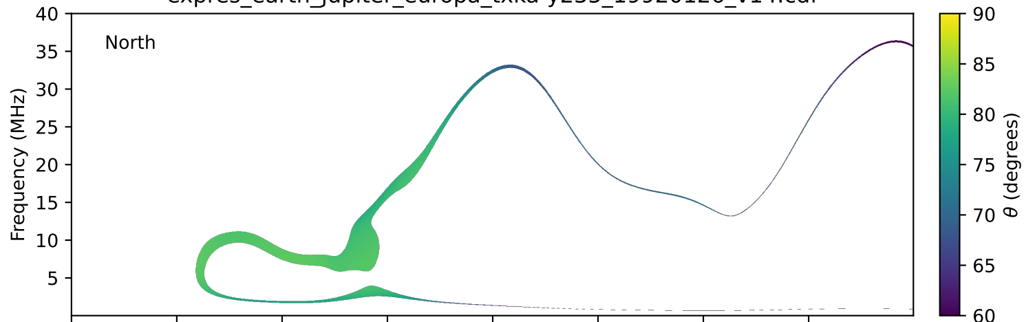
expres_earth_jupiter_europa_txka-y235_19920126_v14.cdf
