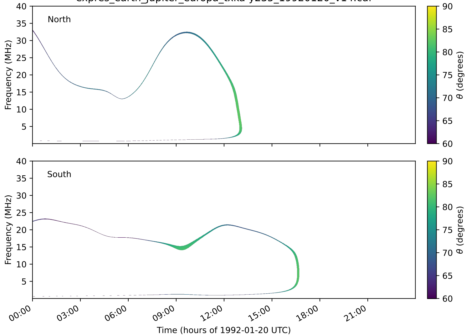
expres_earth_jupiter_europa_txka-y235_19920120_v14.cdf
