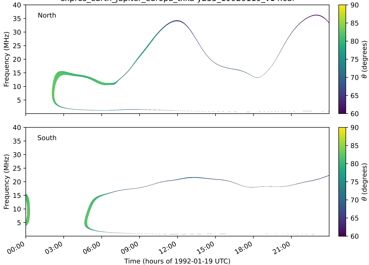
expres_earth_jupiter_europa_txka-y235_19920119_v14.cdf
