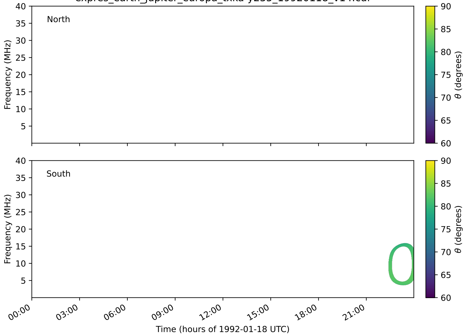
expres_earth_jupiter_europa_txka-y235_19920118_v14.cdf
