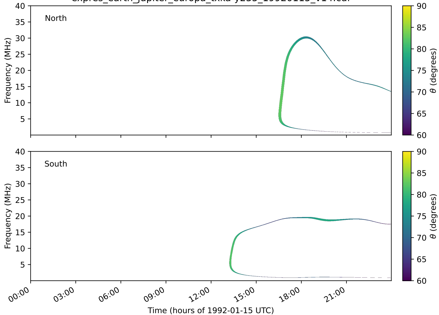
expres_earth_jupiter_europa_txka-y235_19920115_v14.cdf
