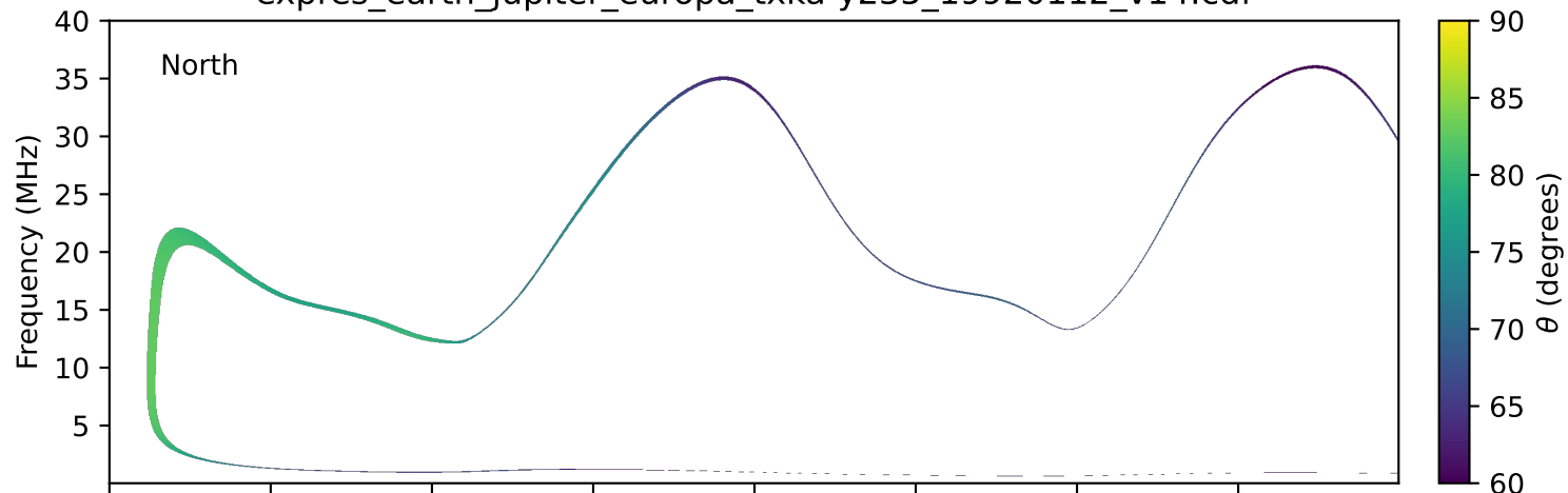
expres_earth_jupiter_europa_txka-y235_19920112_v14.cdf
