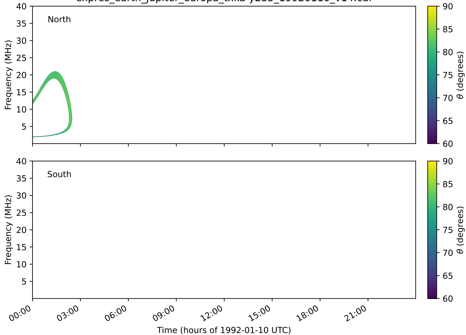
expres_earth_jupiter_europa_txka-y235_19920110_v14.cdf
