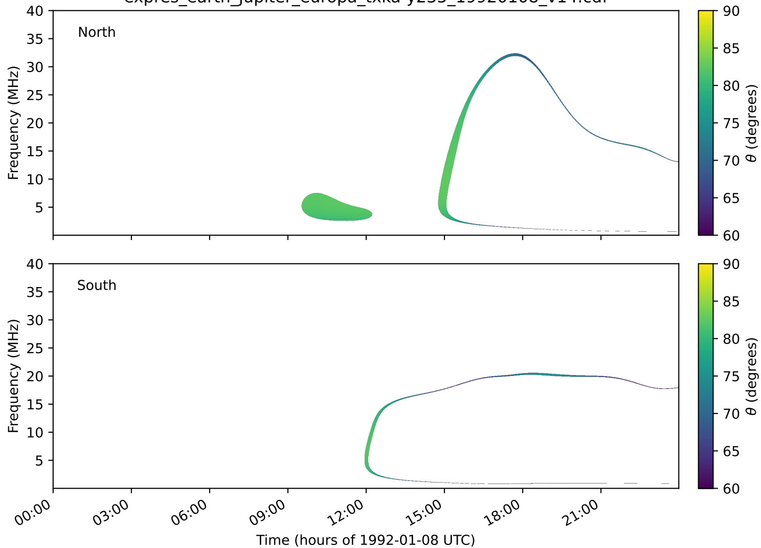
expres_earth_jupiter_europa_txka-y235_19920108_v14.cdf
