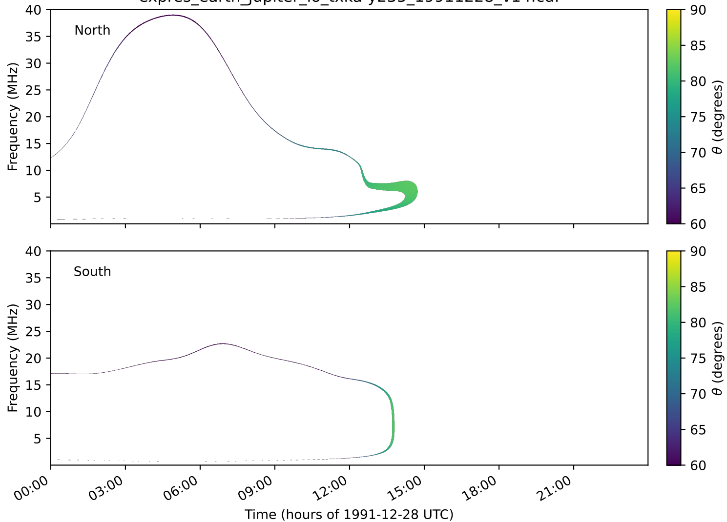
expres_earth_jupiter_io_txka-y235_19911228_v14.cdf
