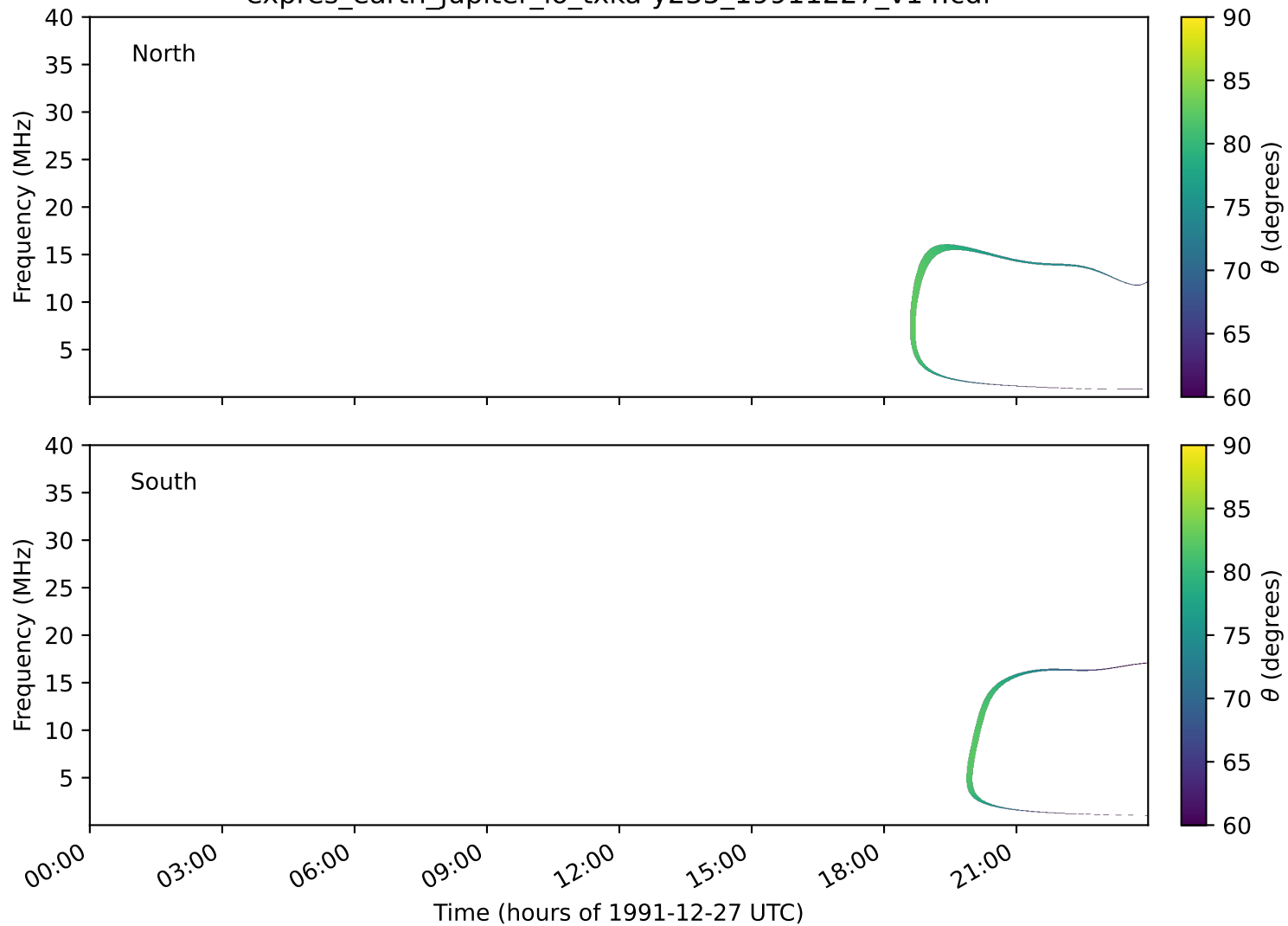
expres_earth_jupiter_io_txka-y235_19911227_v14.cdf
