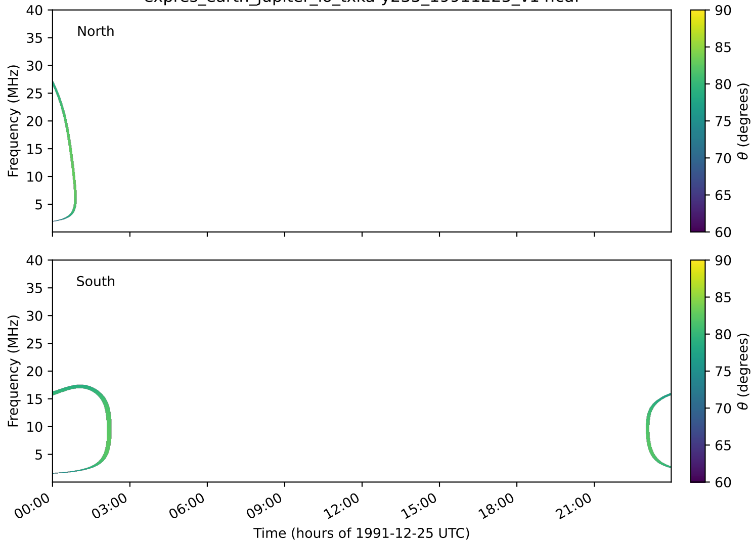
expres_earth_jupiter_io_txka-y235_19911225_v14.cdf
