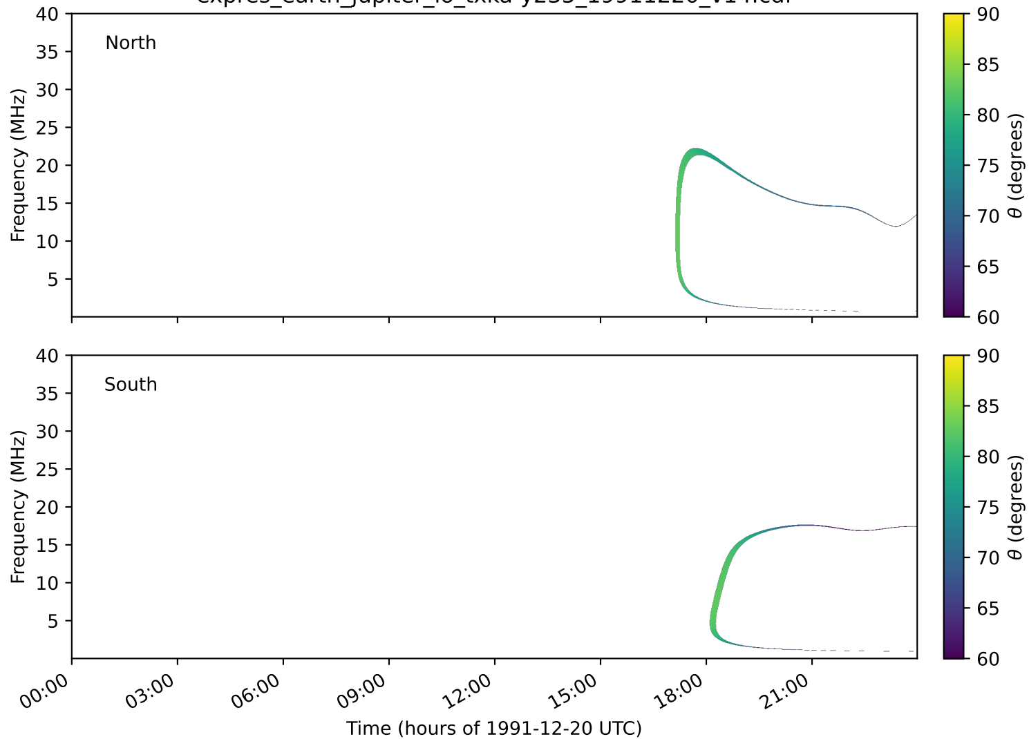
expres_earth_jupiter_io_txka-y235_19911220_v14.cdf
